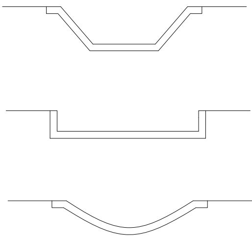
ALTERNATE SECTION A-A
