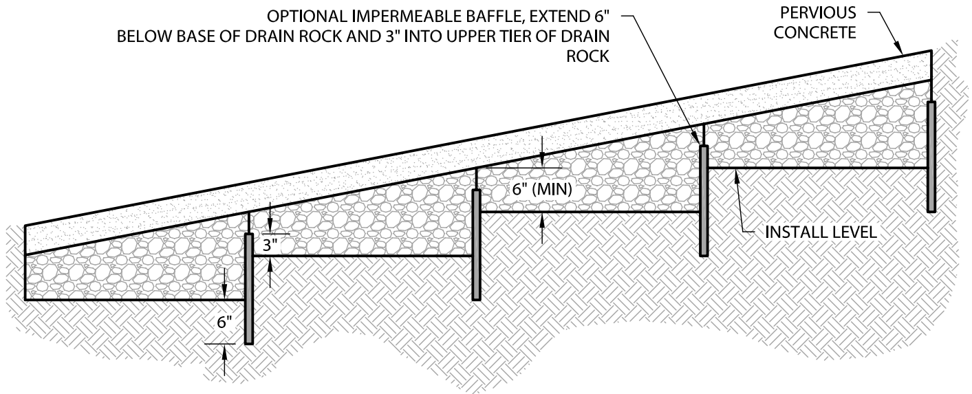
PERVIOUS CONCRETE (ON A SLOPE GREATER THAN 5%)
