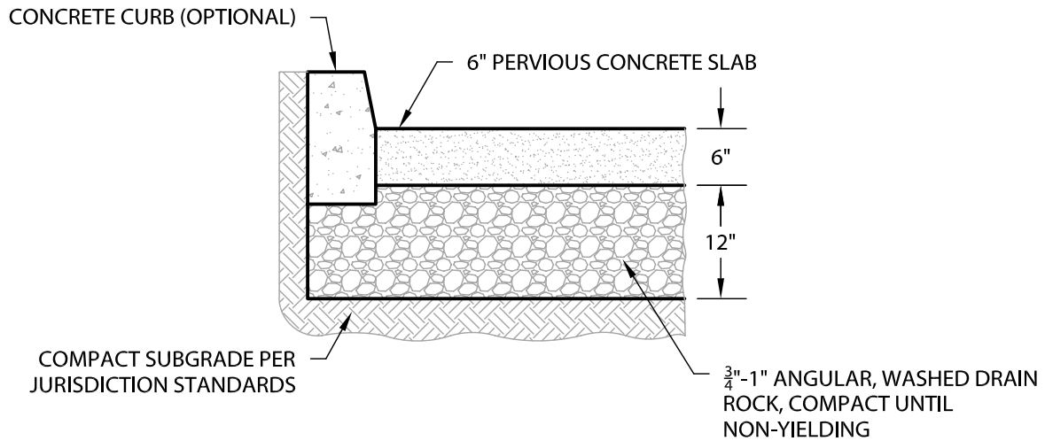
PERVIOUS CONCRETE (ON A SLOPE LESS THAN 5%)
