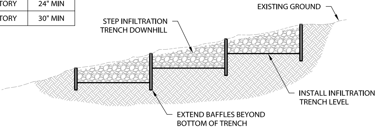
STEP INFILTRATION TRENCH DOWNHILL (ON A SLOPE 5% OR GREATER)
