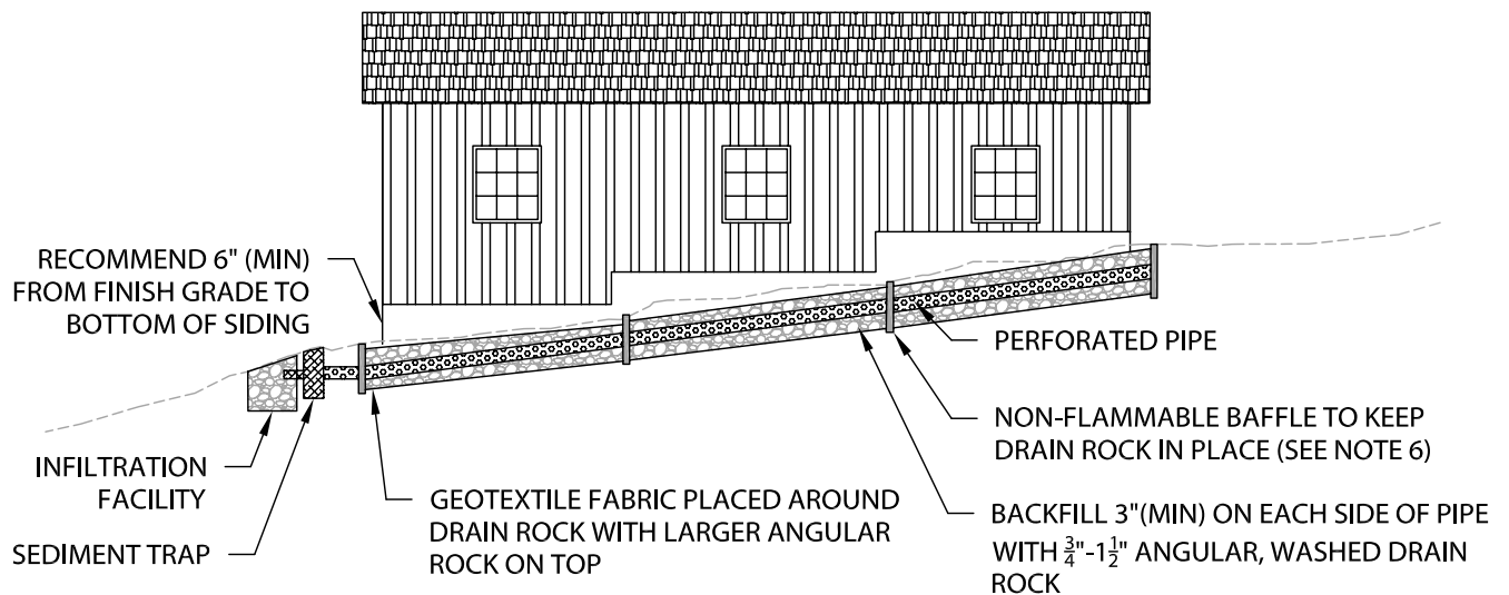
FRENCH DRAIN TO INFILTRATION FACILITY (ON A SLOPE) USED WHEN WATER NEXT TO FOUNDATION MAY BE A PROBLEM
