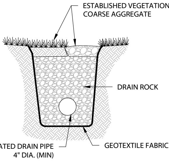
ROCK ARMORED CATCHMENT CONVEYANCE SYSTEM
