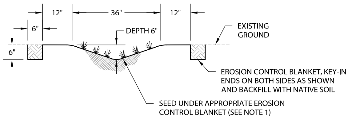
(A-A) TYPE 1 - 2% (MAX) SLOPE
