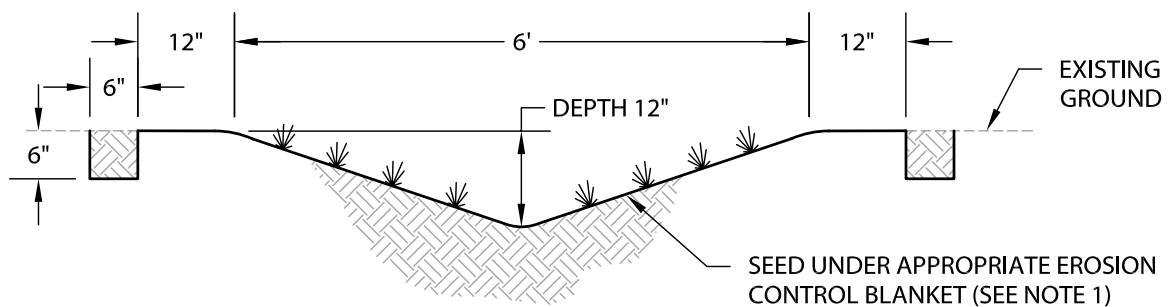
(A-A) TYPE 2 - 3% (MAX) SLOPE
