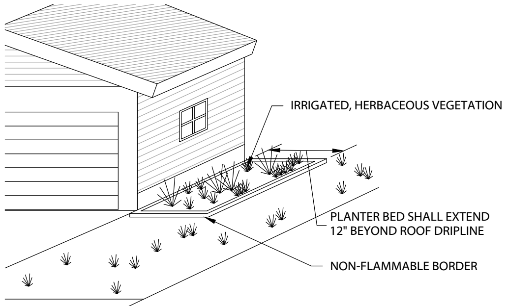
AT GRADE PLANTER BED
