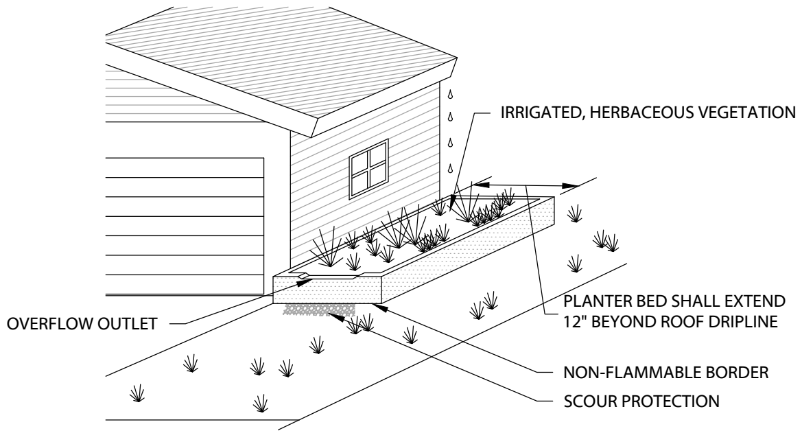
RAISED PLANTER BED
