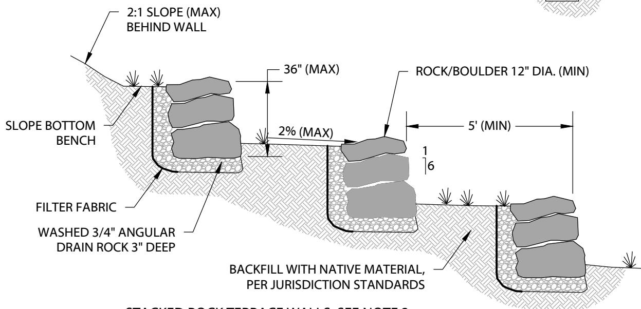
STACKED ROCK TERRACE WALLS. SEE NOTE 3
