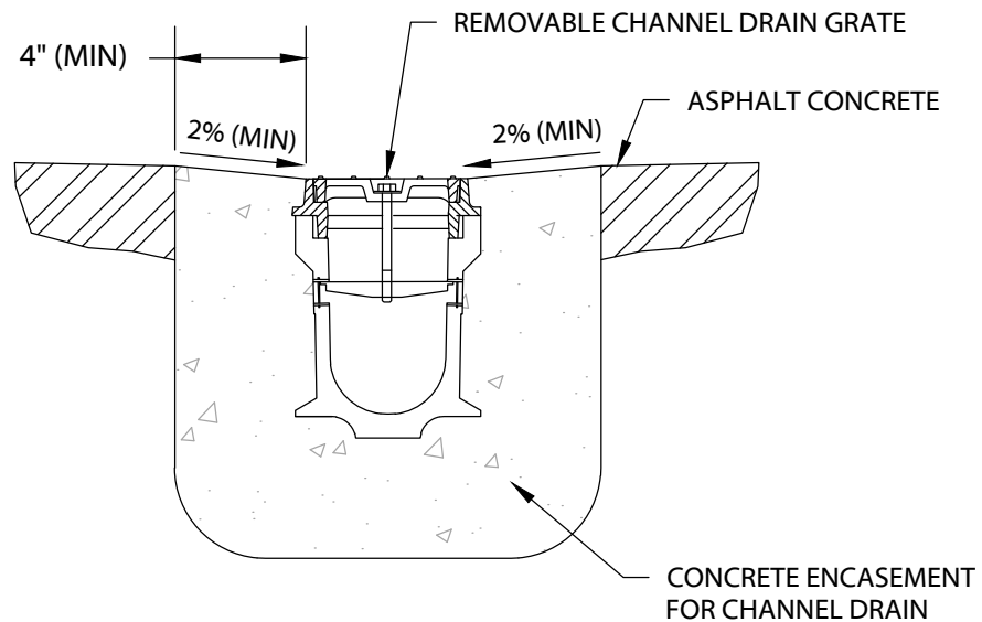
SLOTTED CHANNEL DRAIN SECTION
