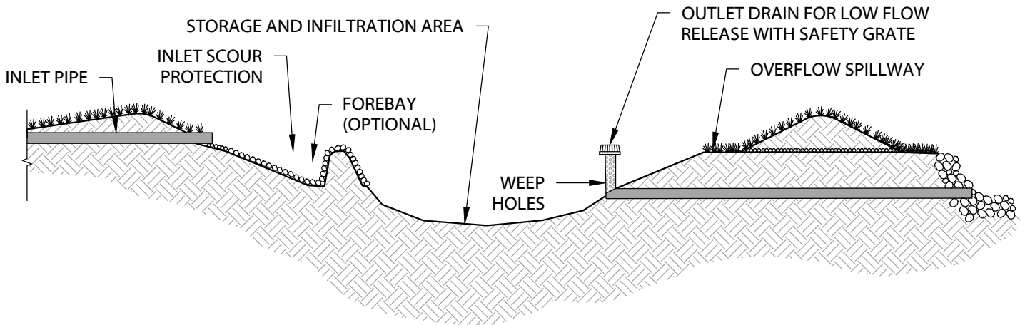
SECTION VIEW
